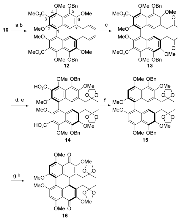
Scheme 4. Reagents and conditions: a) \text{PhI}(\text{OCOCF}_3)_2 , (\text{CF}_3)_2\text{CHOH} ; then aq NaOH, 73%; b) \text{BnBr} , n\text{Bu}_4\text{NI} , NaH, DMF, 78%; c) \text{PdCl}_2 , CuCl, \text{H}_2\text{O} , DMF, 75%; d) \text{H}(\text{OEt})_3 , \text{HOCH}_2\text{CH}_2\text{OH} , cat. TsOH, 90%; e) NaCN, DMSO, \text{H}_2\text{O} , 110°C, 100%; f) \text{Pd}(\text{OCOCF}_3)_2 , \text{Ag}_2\text{CO}_3 , 5% DMSO/DMF, 70°C; then \text{NaBH}_4 , 60%; g) \text{H}_2 , Pd/C, MeOH, 100%; h) \text{MnO}_2 , NaOH, THF, EtOH, 88%. Bn = benzyl, DMSO = dimethyl sulfoxide, Ts = para -toluenesulfonyl.
